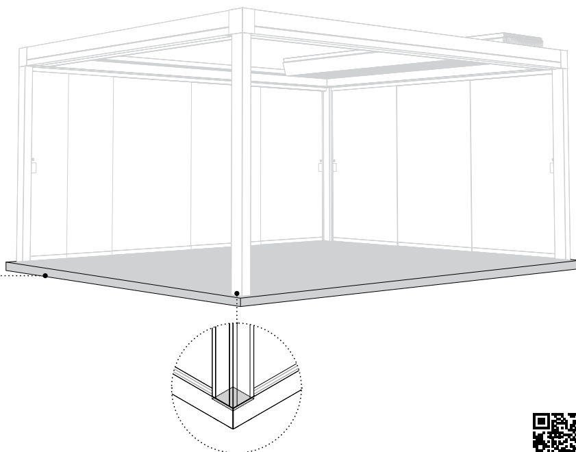
Staffa a terra del montante a scomparsa Ground bracket for concealed posts
